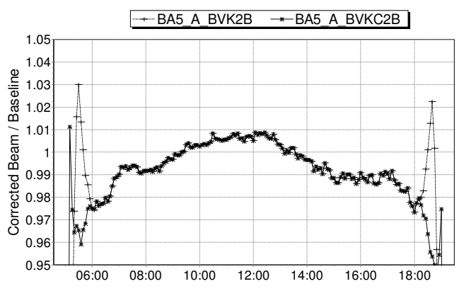
Figure 7: Corrected Direct Beam With and Without Cat Ear Correction
