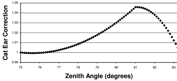
Figure 3: Cat Ear Correction
