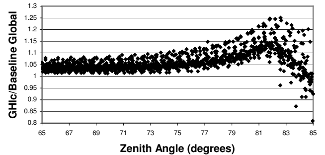
Figure 2: NREL GHI_c /Base Line Global from 65-85° Zenith Angle: The Cat Ear Error.
