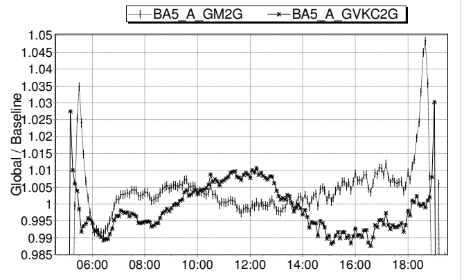
Figure 5: GM2G and GVKC2G on a Typical Clear Day
