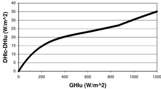
Figure 1: Diffuse Correction, DHI_c - DHI_u
