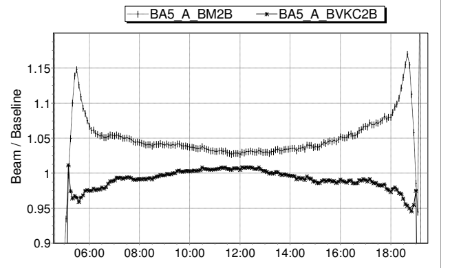
Figure 6: BM2B and BVKC2B on a Typical Clear Day
