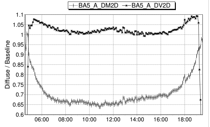
Figure 4: DM2D and DV2D on a Typical Clear Day
