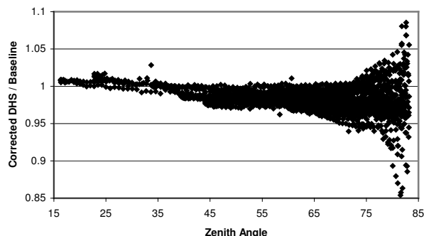
Figure 9: Corrected Direct Beam Projected on a Horizontal Surface Divided by Baseline Over a Range of Zenith Angles
