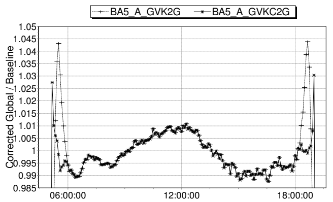
Figure 8: Corrected Global With and Without Cat Ear Correction
